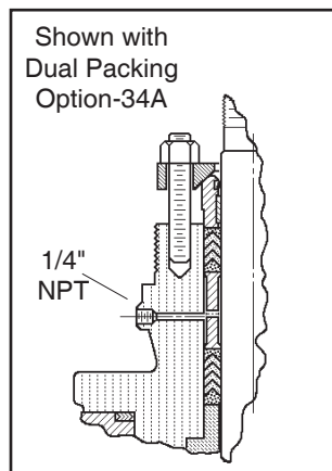
FIGURE 4 Leak-Off Conn. Option-26
