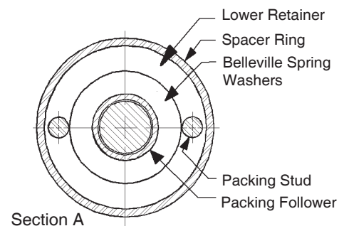
FIGURE 3 External Live-Loaded Packing Details
